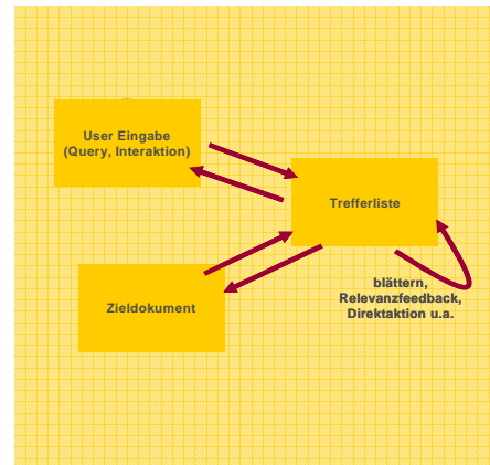
User Interface
